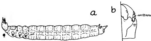
Fig. 321. a, Chaetartria seminulum Herbst. (Redrawn from Boving & Craighead); b, Dorsal aspect of a half head.
